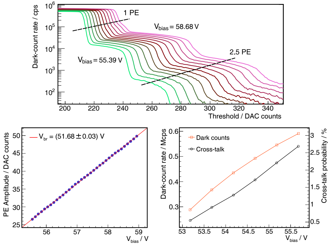
Figure 3: (Top) Dark-counts per second (cps) as a function of the discriminator threshold at different V_{\text{bias}} . The dark-count rates and PE amplitudes shift towards higher values when rising the V_{\text{bias}} . (Bottom-left) V_{\text{br}} determination for an individual SiPM. The linear extrapolation to 0 amplitude yields the value of V_{\text{br}} . (Bottom-right) Dark-count rate (red squares) and cross-talk (black dots) as a function of the V_{\text{bias}} .
